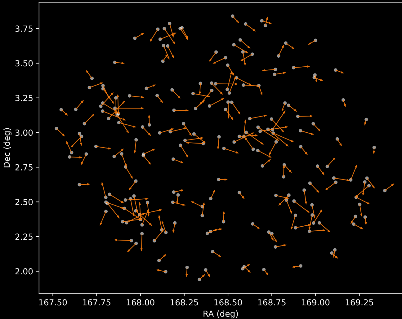
GALAH DR4 Cluster 2 Proper Motion Vectors (n=198)
