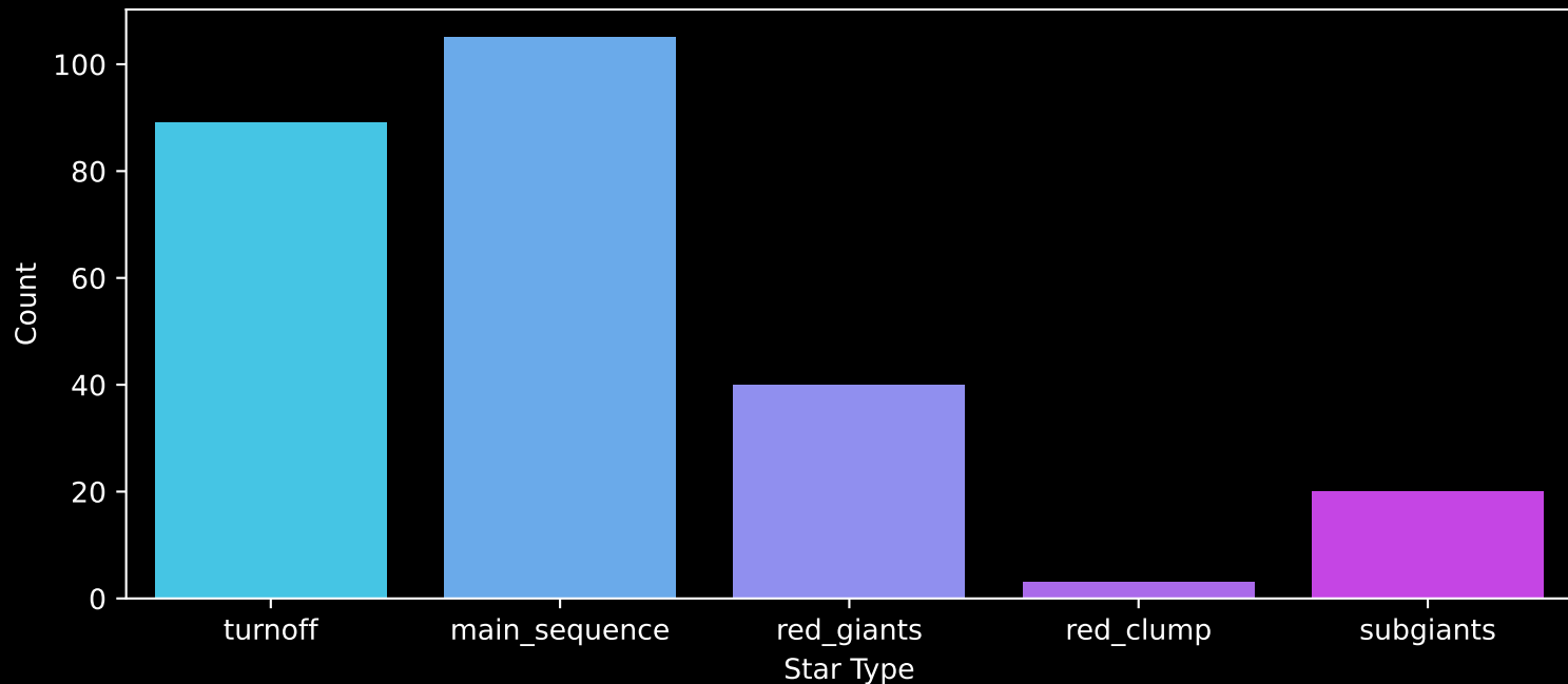
GALAH DR4 Field: [1107] Count plot of Star Type
