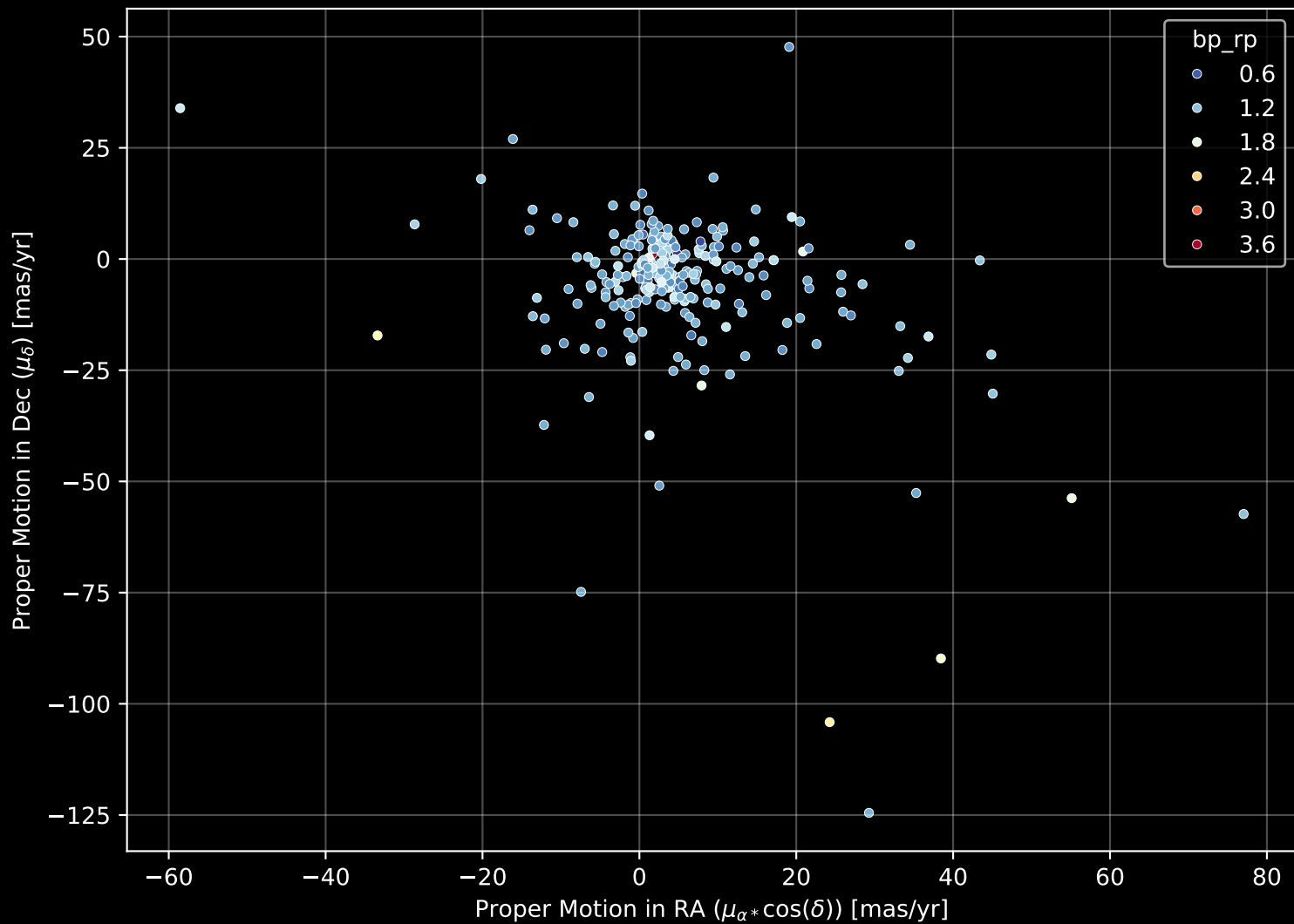
GALAH DR4 Field: [1107] Proper Motion Diagram (n= 257)
