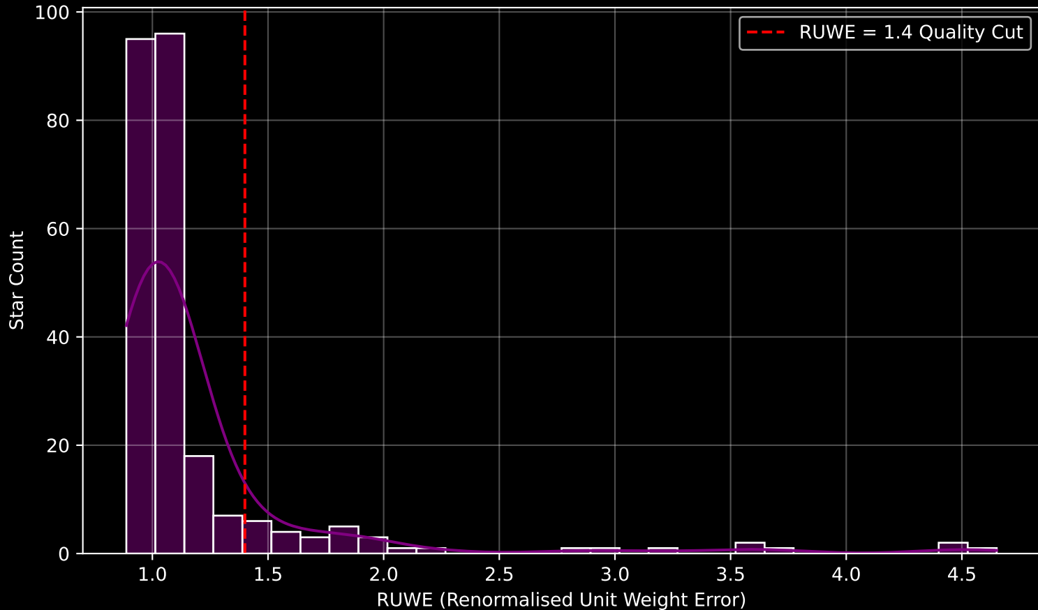
GALAH DR4 Field [1107] RUWE Distribution (n= 248)
